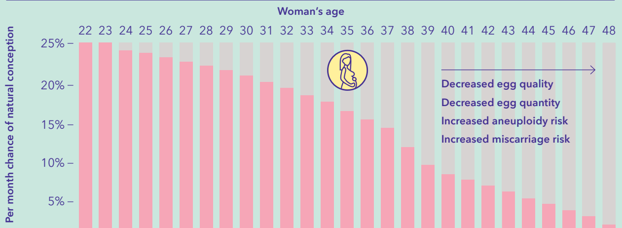
Monthly chance of natural conception
