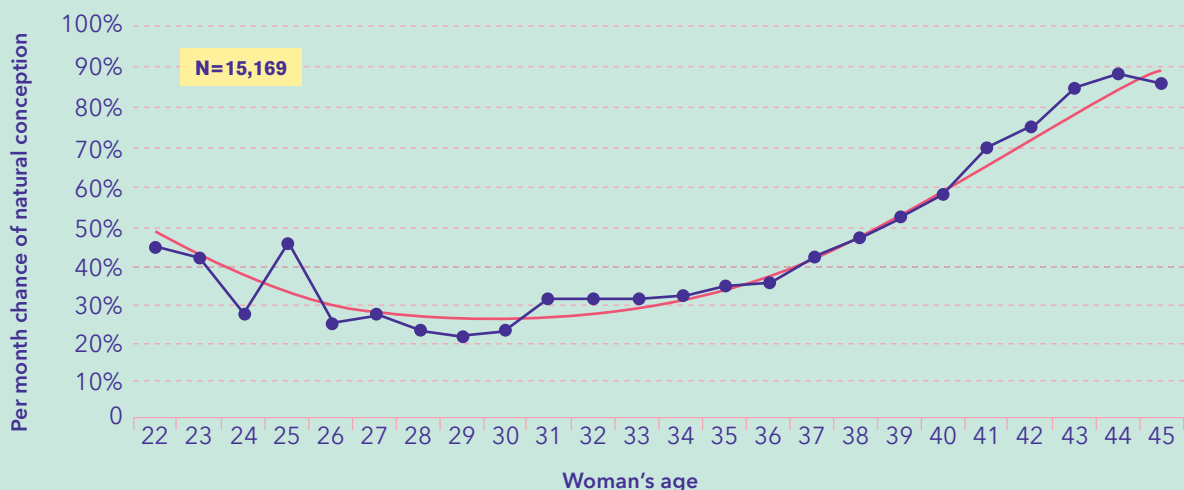
Maternal age and prevalence of aneuploidy
